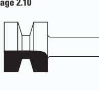
HW WEDGE TONGUE AND GROOVE BITS Z=2 Page 2.11
