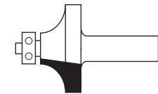
HW CORNER ROUNDING BITS WITH BALL BEARING GUIDE Z=2 Page 2.19
