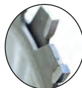
Scoring sawblades for cutting laminated materials
